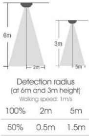
Detection Range
